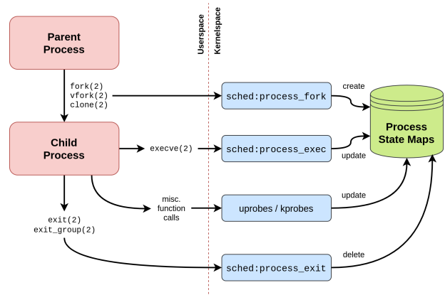
Figure 2: The various mechanisms that bpffox uses to manage process state. Probes marked sched:* are tracepoints instrumenting scheduler events in the kernel. Uprobes and kprobes instrument userspace and kernelspace function calls respectively.
