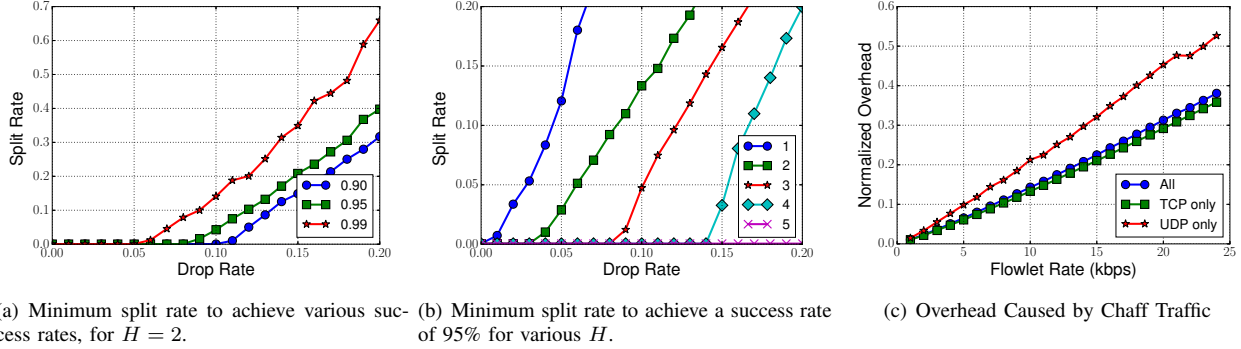
Figure 5. (a) and (b) show the minimum packet splitting rate required to achieve a certain success probability, given a certain failure counter H (Section 4.2). In (a), H = 2 , with success rates of 90%, 95%, and 99%; in (b), the required success rate is 95%, and H \in \{1, \dots, 5\} . (c) Bandwidth overhead caused by added chaff traffic for traffic shaping. We normalize the overhead by dividing the added overhead by the original bandwidth. Lower is better.
