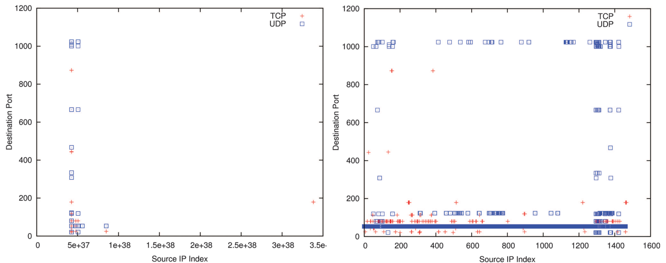
Figure 3: These graphs display the data set of Section 'IPv6 – only data set' (destination ports contacted by each source IPv6 host) before (left) and after (right) indexing the source IPv6 address and removing unused address space. The graph on the right uses an index value in place of the absolute IP address.
