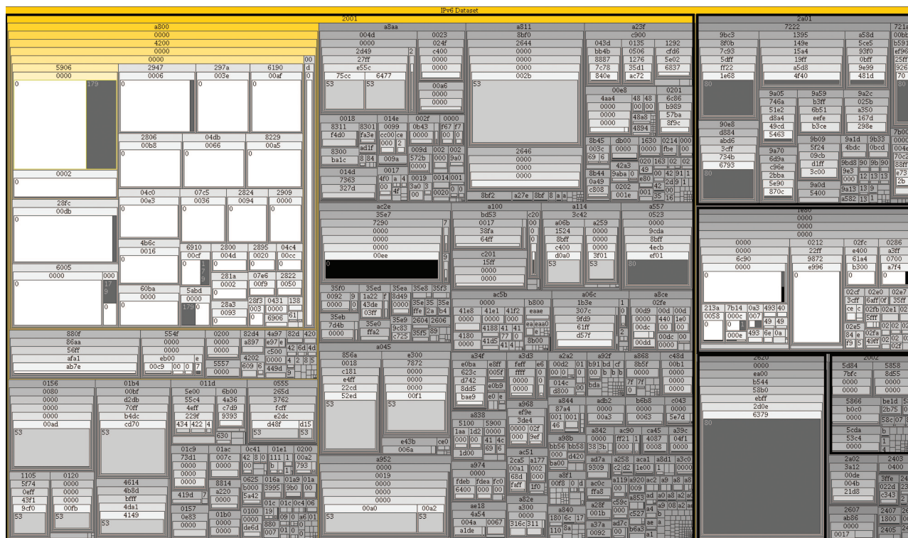
Figure 5: A treemap representing IPv6 source address, destination port and packet count (ICMP (white), TCP (dark grey), UDP (light grey), everything else (black)). Best viewed in color. Full resolution version available at: http://bit.ly/vizsec1 .
