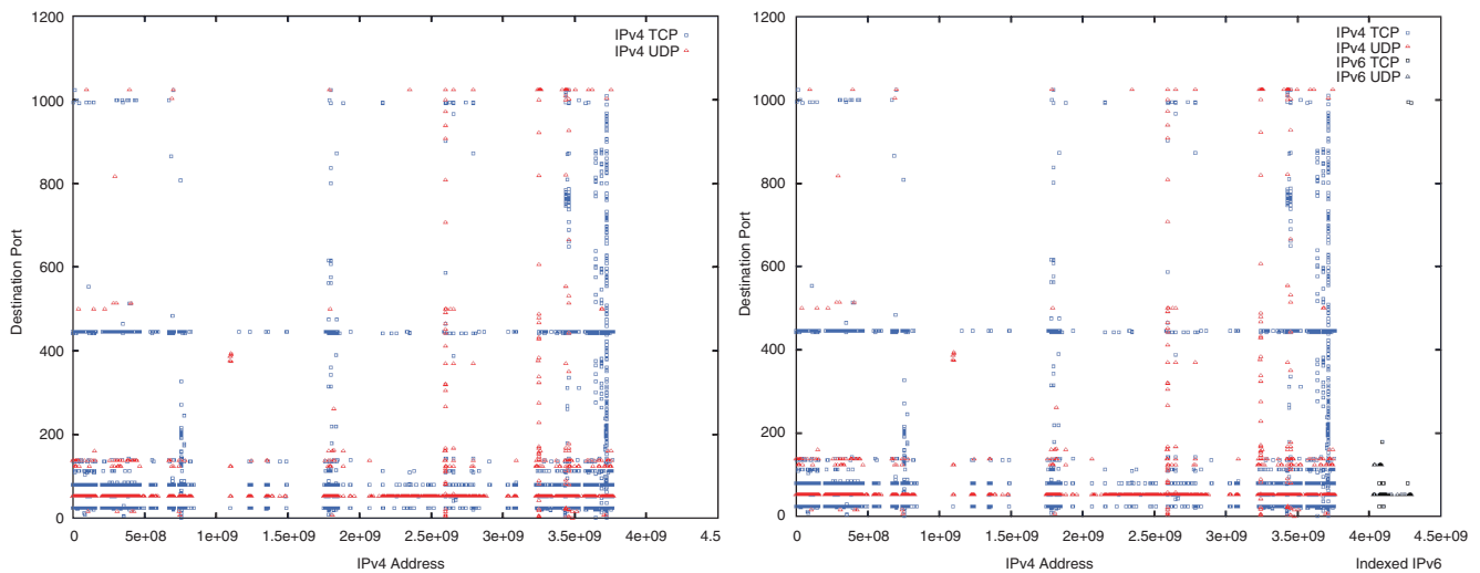
Figure 4: The graph on the left plots destination ports contacted only by IPv4 hosts in the dual-stack data set of Section 'Dual-stack data set'. The graph on the right maps IPv6 hosts into the unused portion of the graph, displaying the full data set.
